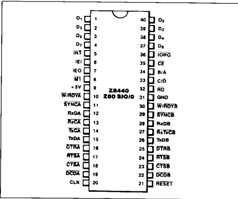
Figure 6 : Z80 SIO-0 Dual in Line Pin Configuration.
